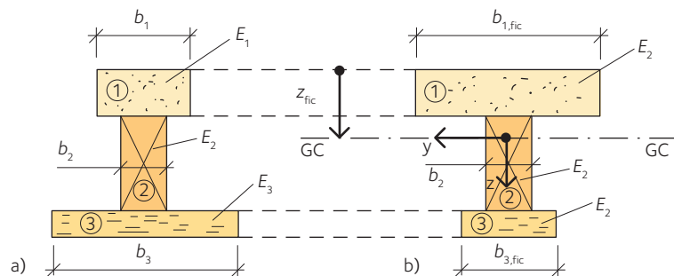
Figure 5.4 Going for a fictitious or transformed cross-section a) The real physical cross-section, b) fictitious cross-section drawn to scale, if part 2 is taken as reference with E_1 = 2, E_2 och E_3 = E_2/2 .
