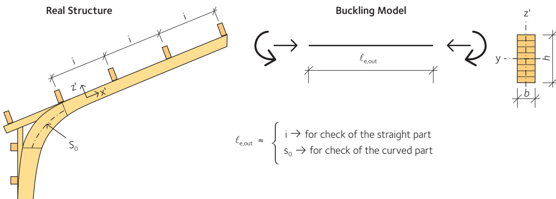
Figure 3.18 Buckling lengths for out-of plane buckling of a portal frame
