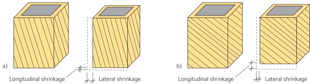
Figure 2.11 Diagrammatic sketch of micro fibril arrangement and shrinkage in normal wood and in compression or juvenile wood. Note the difference in micro fibril angles. a) Shrinkage at normal micro fibril angle. b) Shrinkage at large micro fibril angle (compression wood or juvenile wood).
